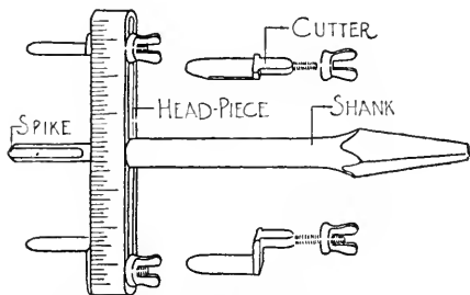
FIG. 103. WASHER CUTTER.
